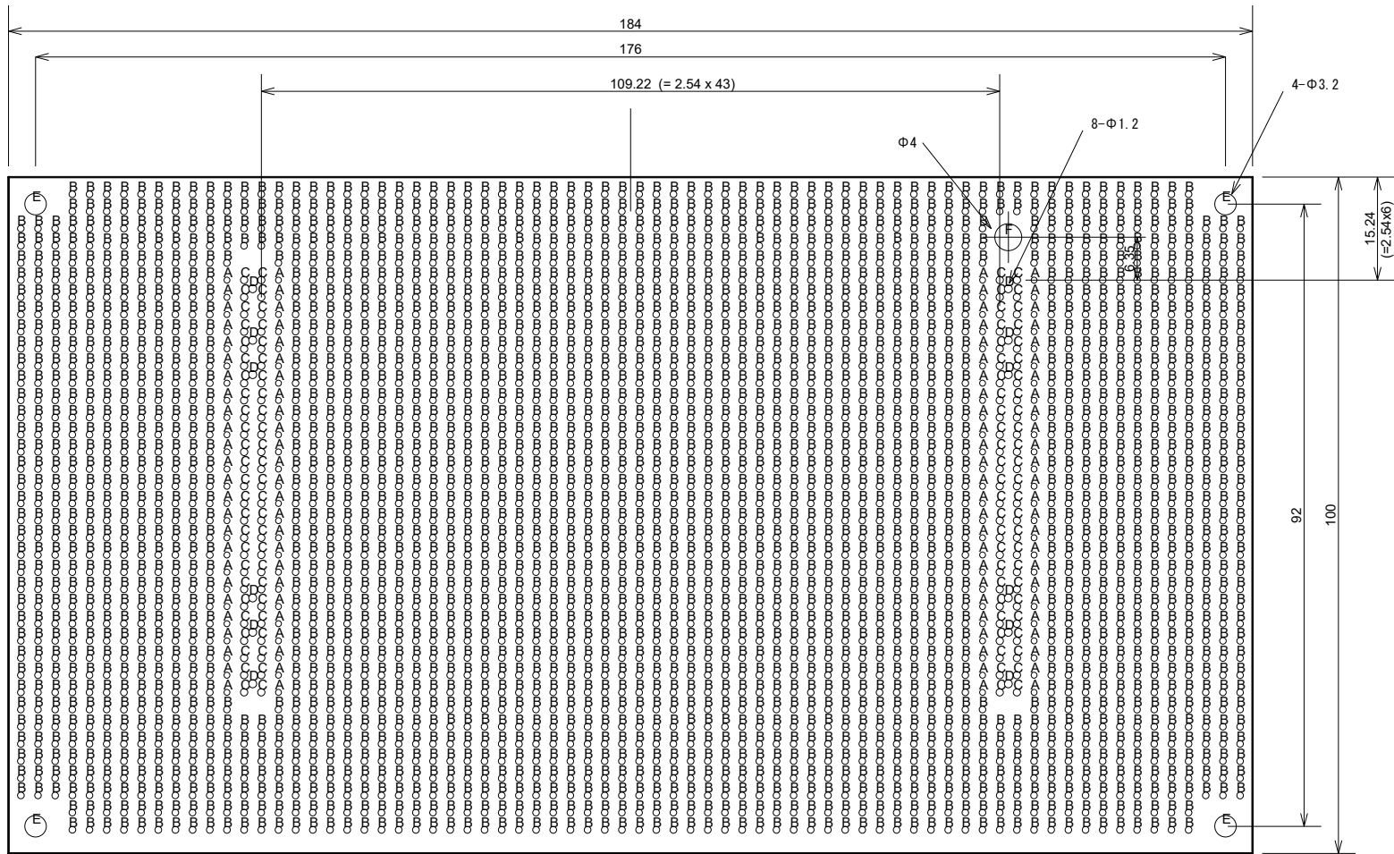
55 PCB DIMENSION
