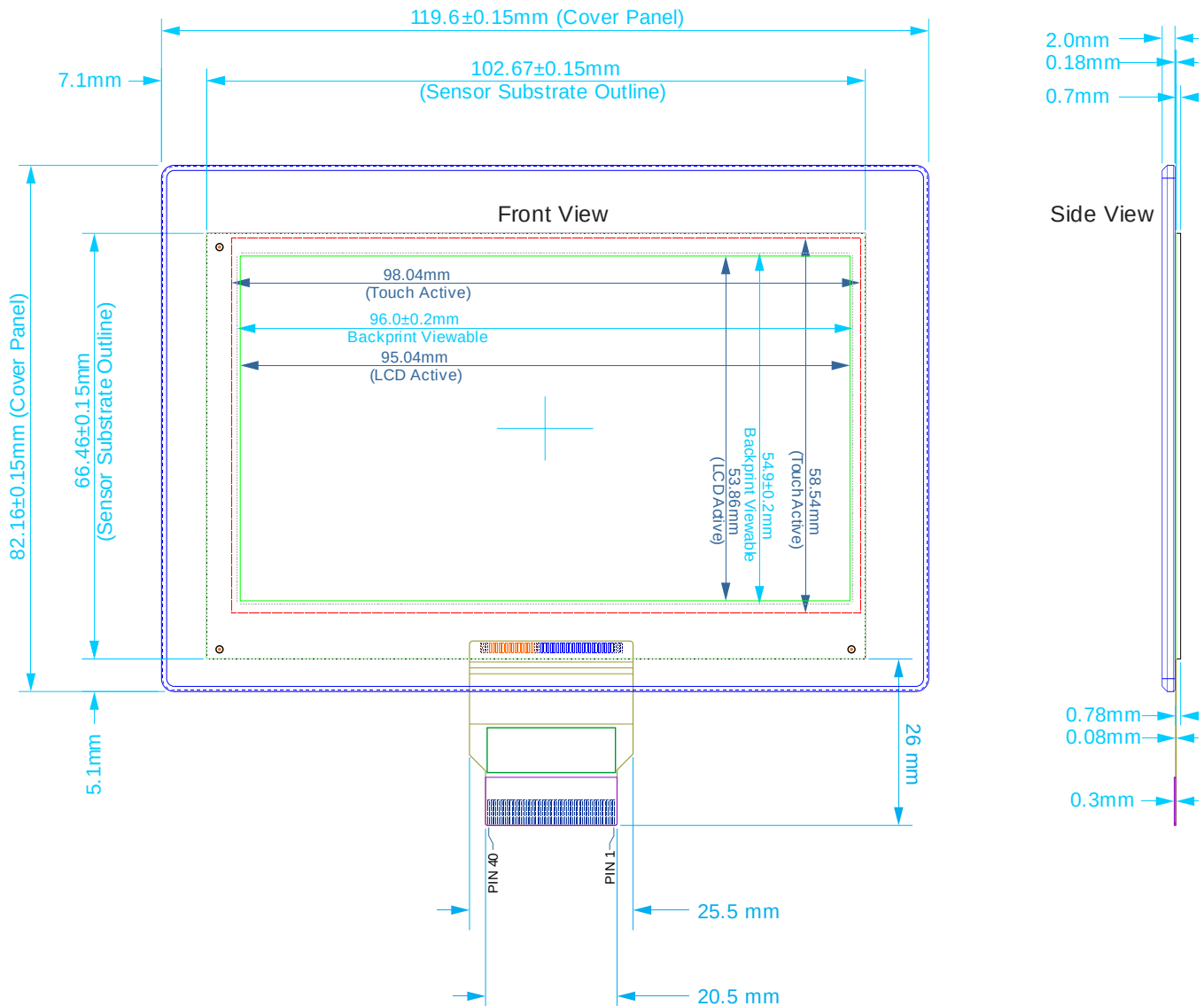
Figure 4 - Sensor Only Dimensions
