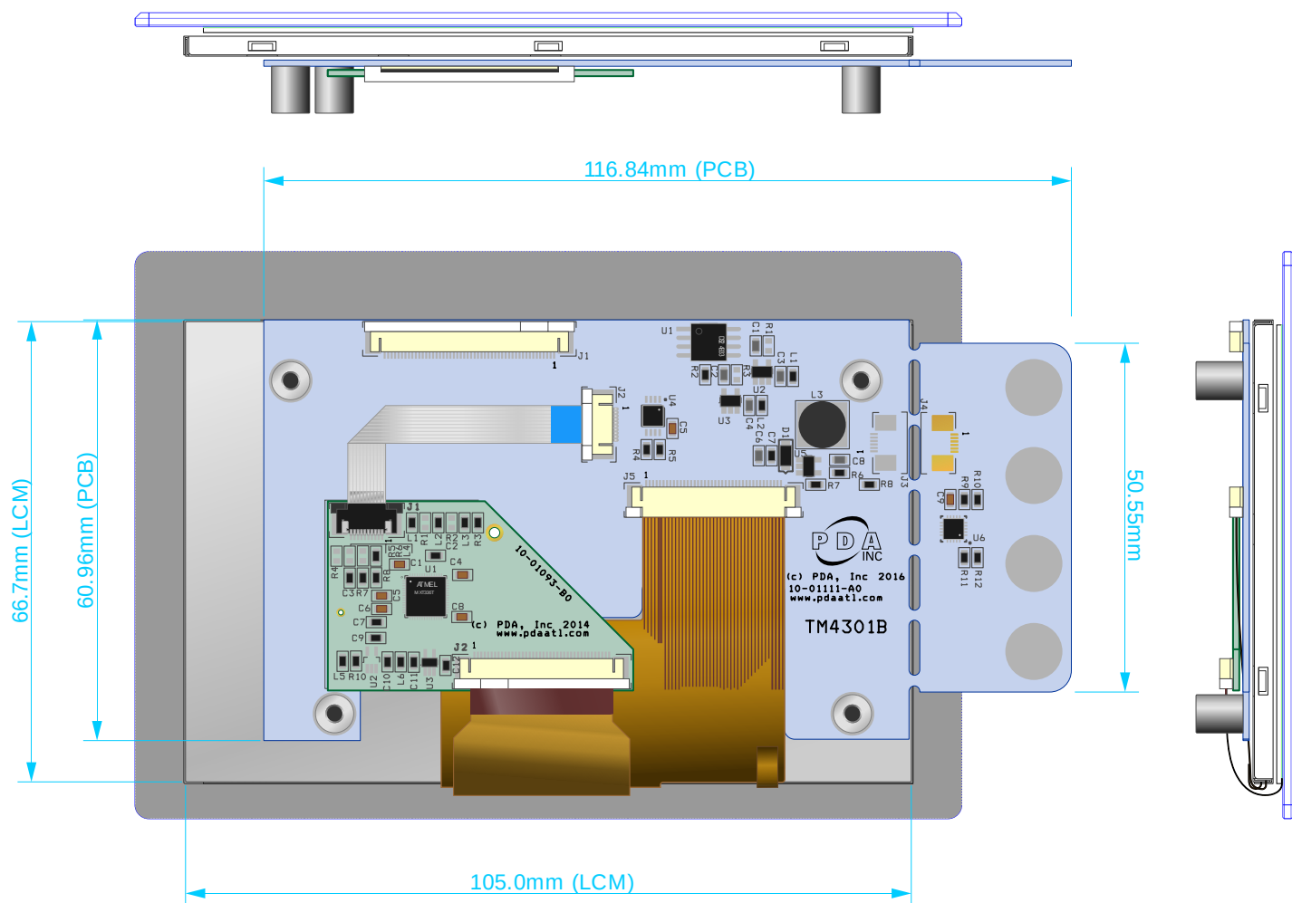
Figure 5 – Module Dimensions
